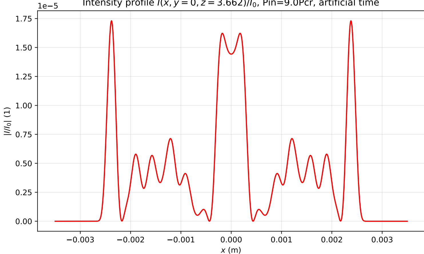
Intensity profile I(x, y = 0, z = 3.662)/I_0 , P_{in}=9.0P_{cr} , artificial time
